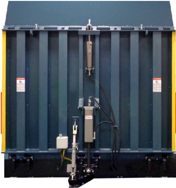
* VSH Series, 6' x 5', 40,000 CIR, with remote motor shown
