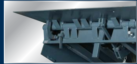
High strength piano hinge construction and lip extension mechanism.
