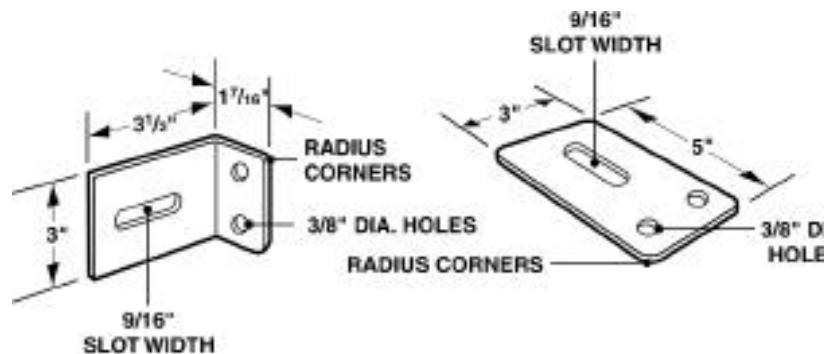
ANGLE AND FLAT MOUNTING BRACKETS
