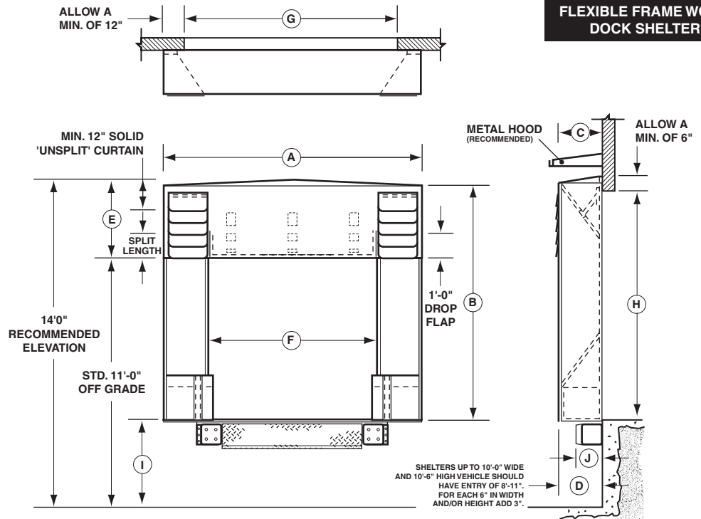
PLAN VIEW
